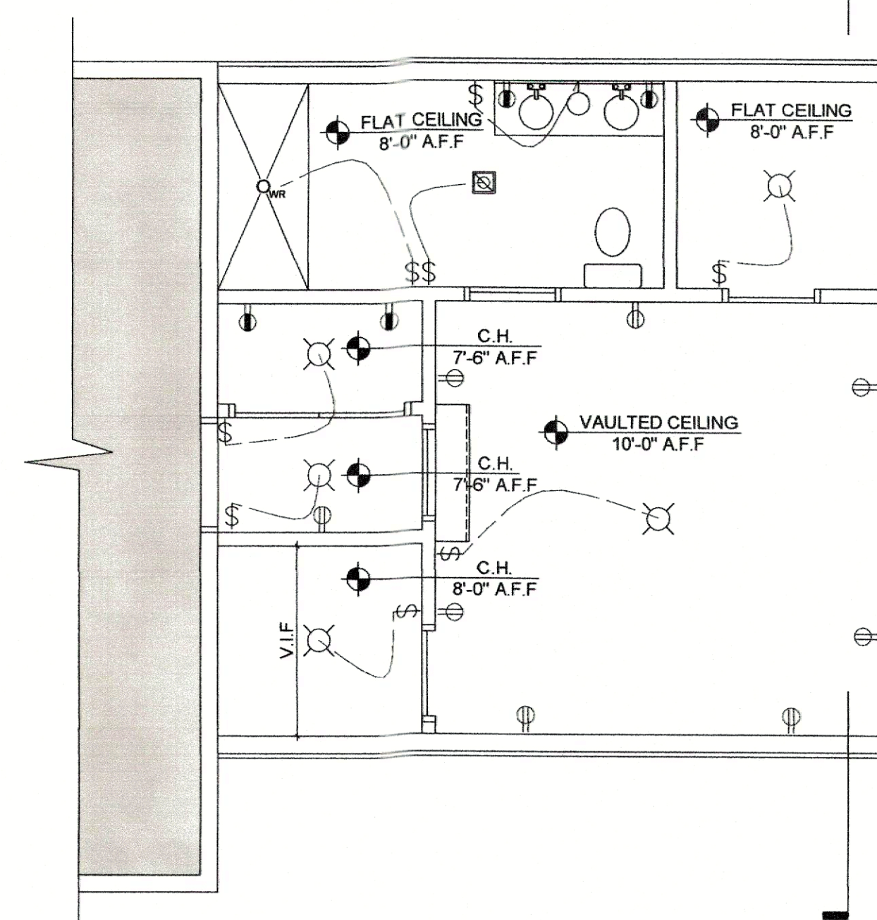
2 Lighting & Electrical Plan 1/4" = 1'-0"
