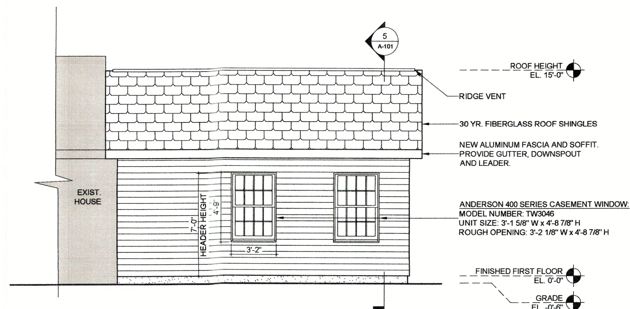
3 Front Elevation 1/4" = 1'-0"
