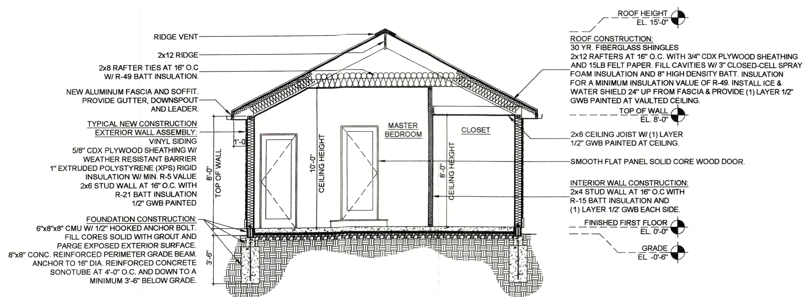
5 Building Section 1/4" = 1'-0"
