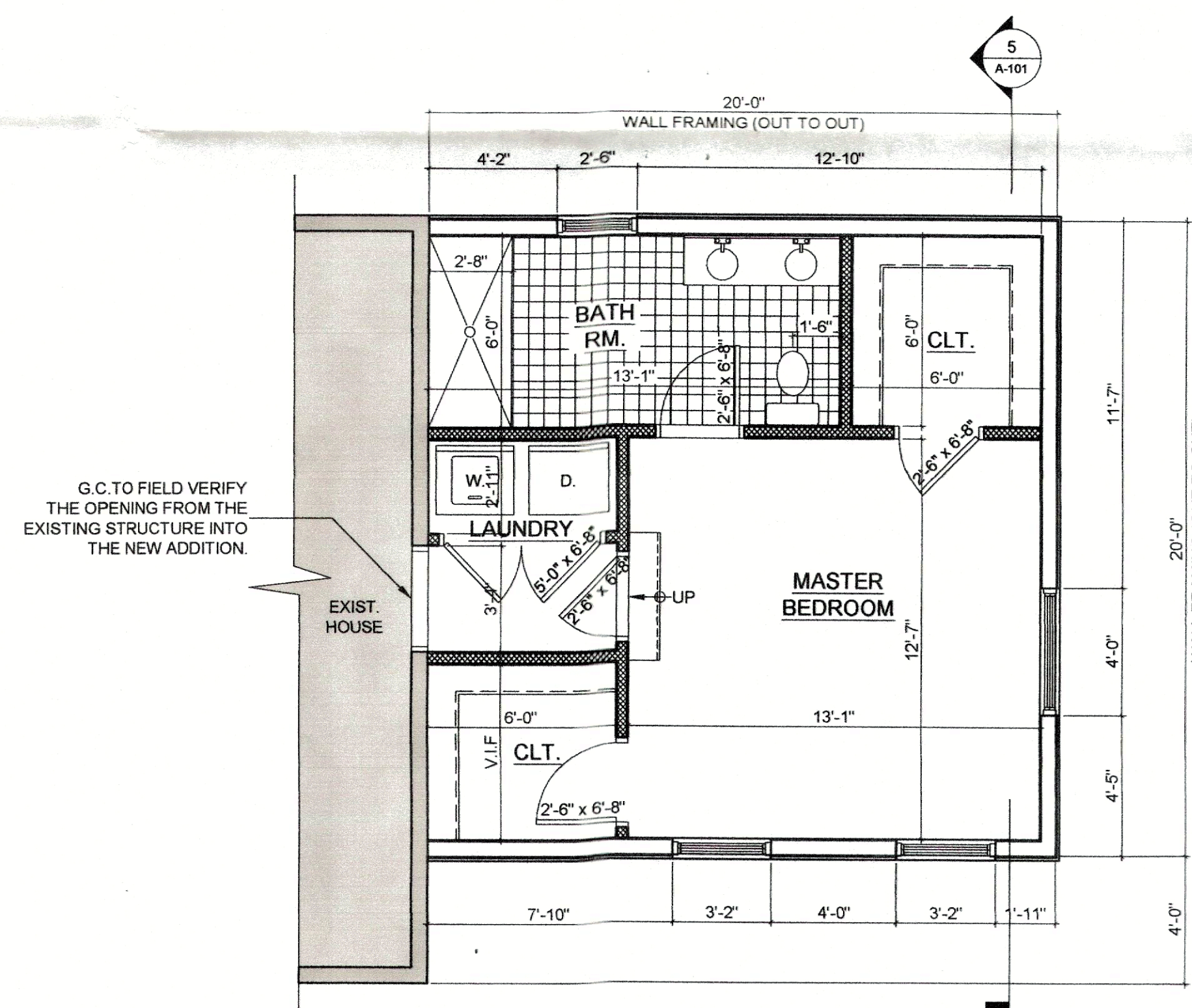
1 1st Floor Plan 1/4" = 1'-0"
