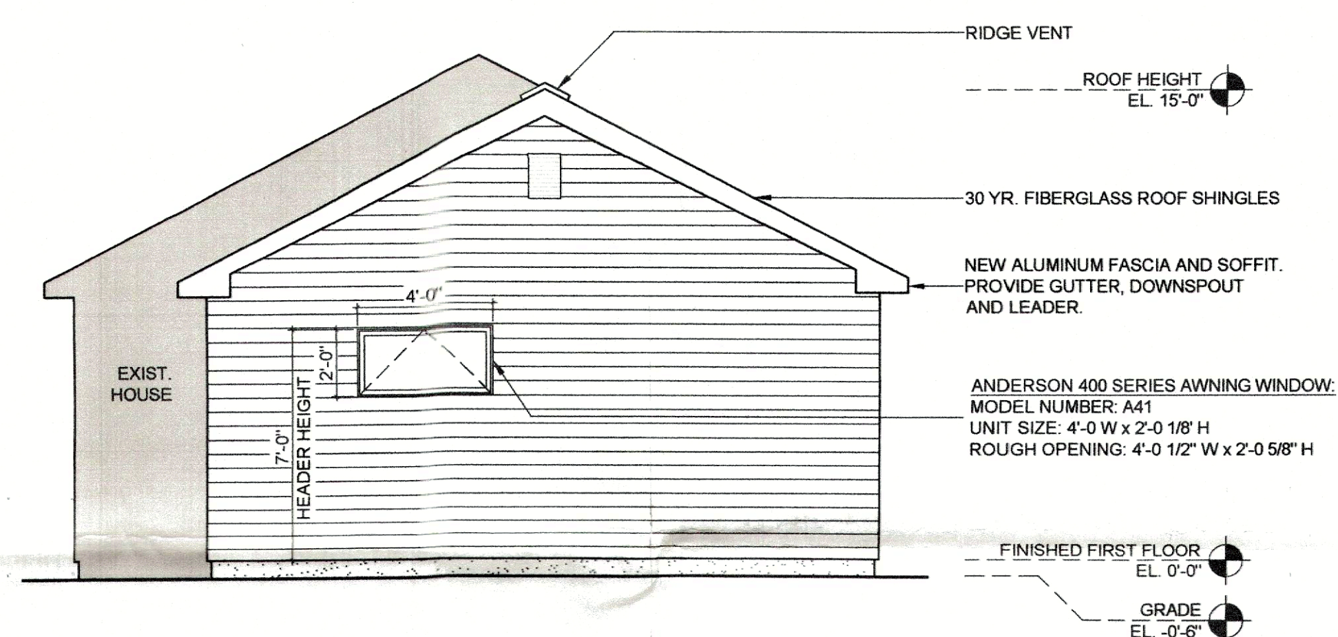
4 Side Elevation 1/4" = 1'-0"
